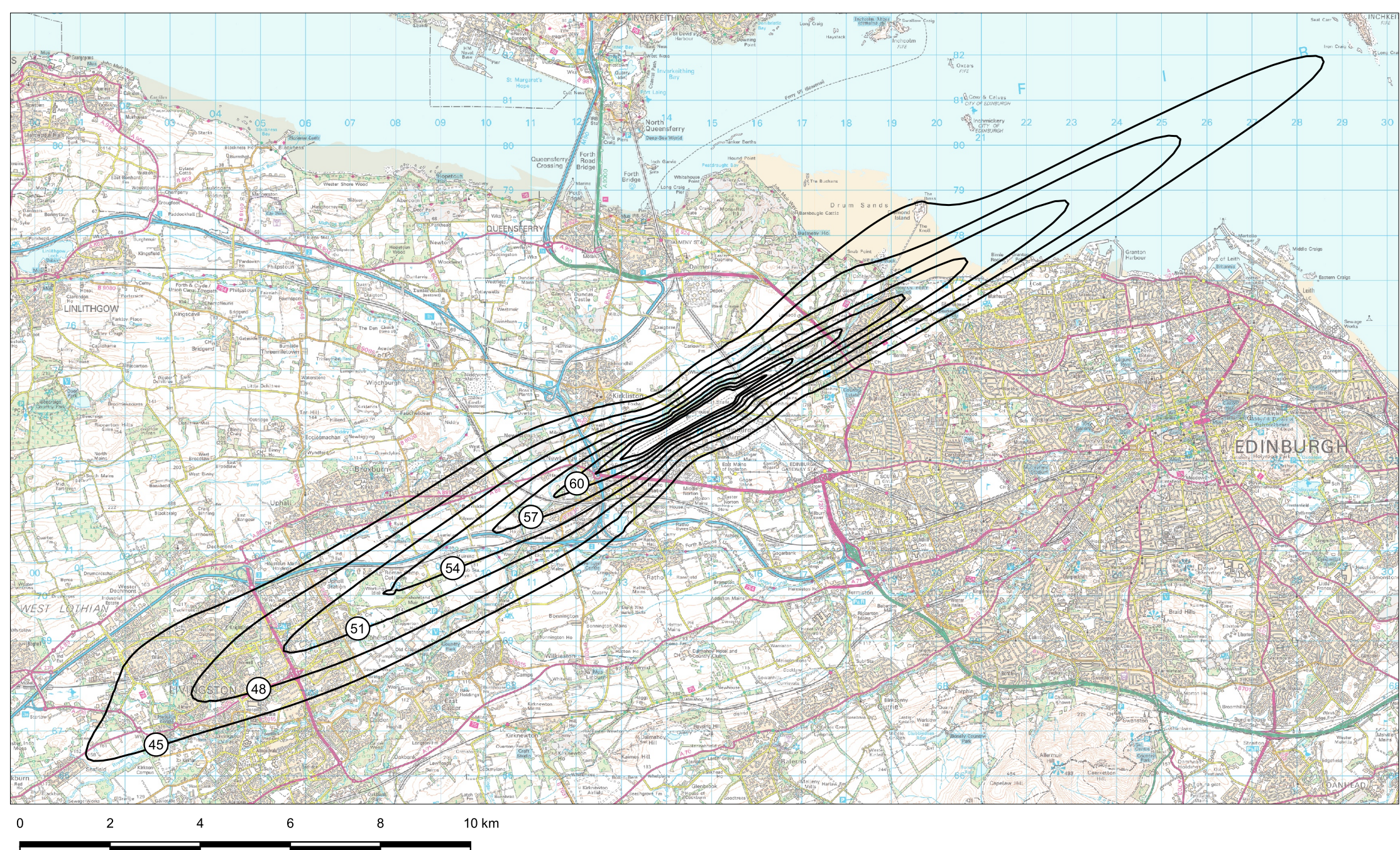
EDINBURGH AIRPORT 2025 Average Summer Night 45-66 dB L_{Aeq,8h} Contours Actual Runway Modal Split 81% W / 19% E
